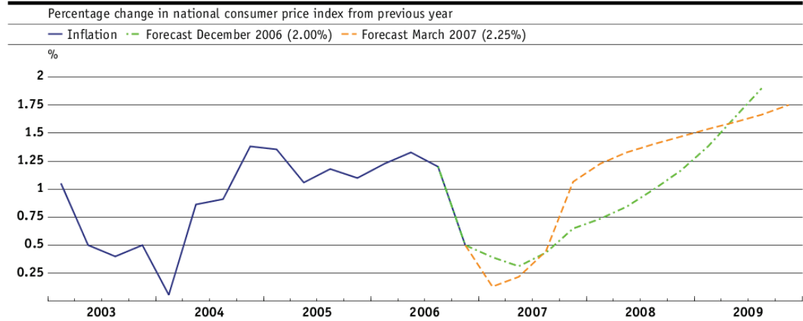
Inflation forecast of December 2006 with Libor at 2.00% and of March 2007 with Libor at 2.25%
