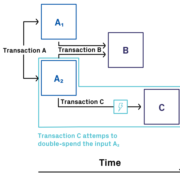
Graph C2: Double-spending attempt
